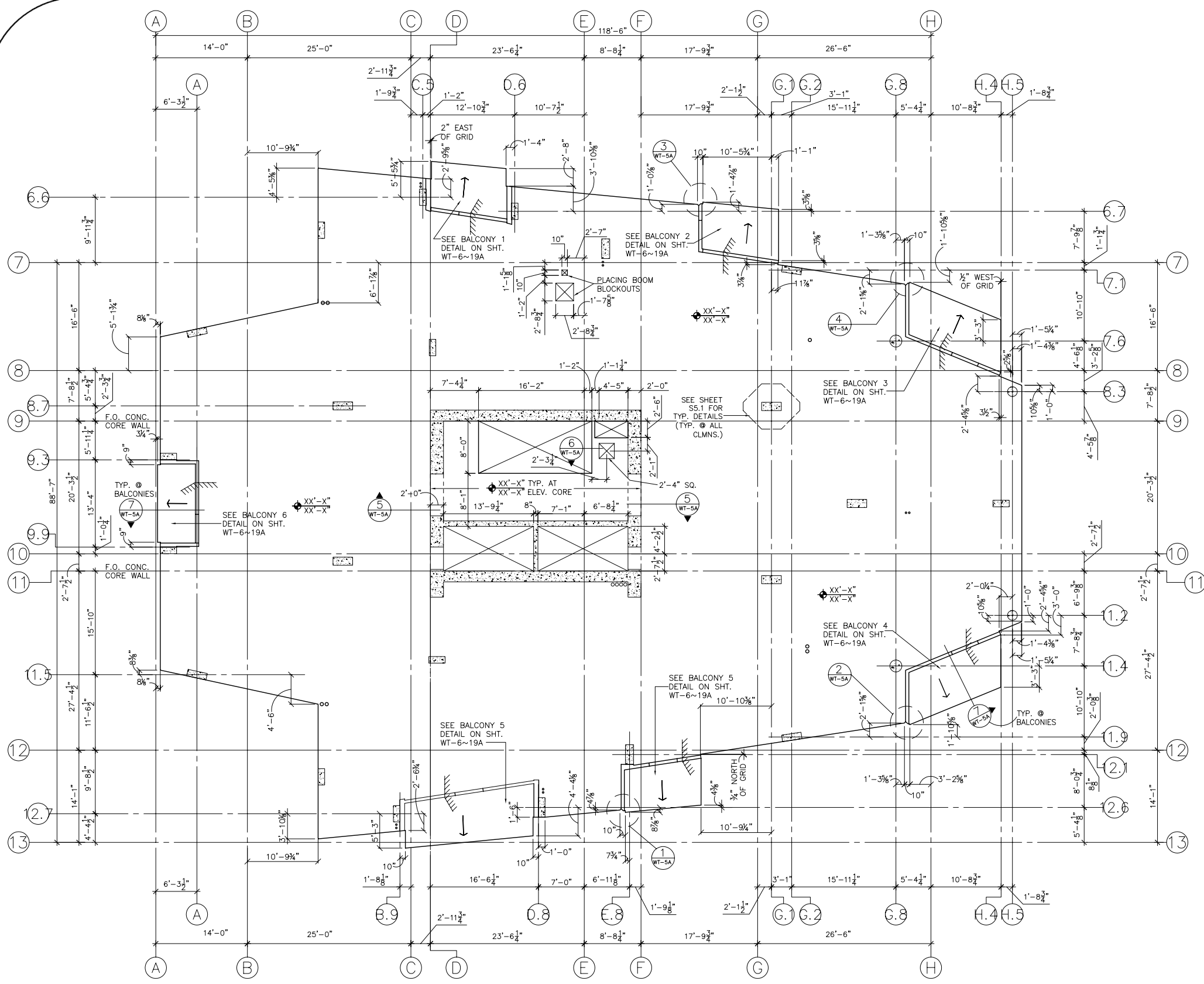
WEST TOWER ~ LEVELS 6 ~ 19 SLAB PLAN 1/8"=1'-0"
